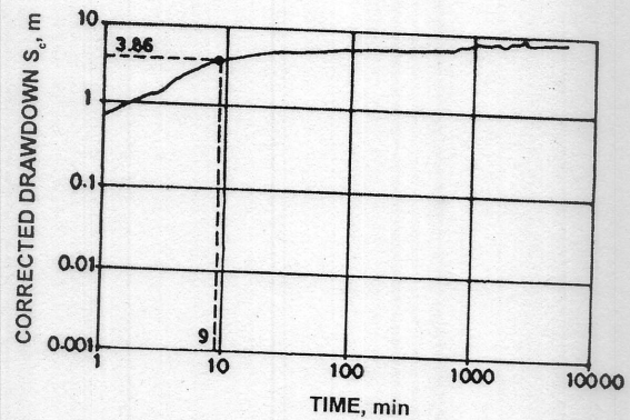
Figure 17 : Typical Result of CD Test
