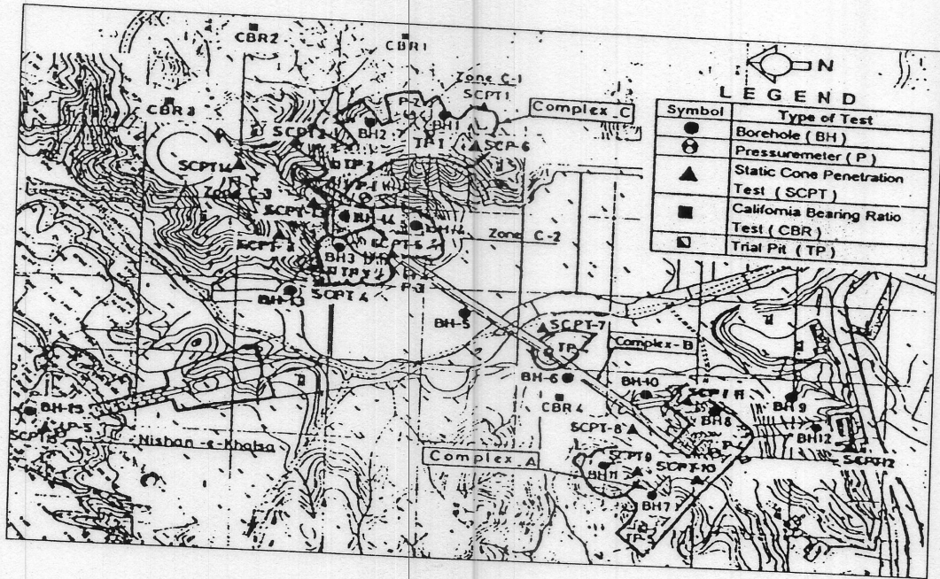
Figure 7 : Layout Plan
