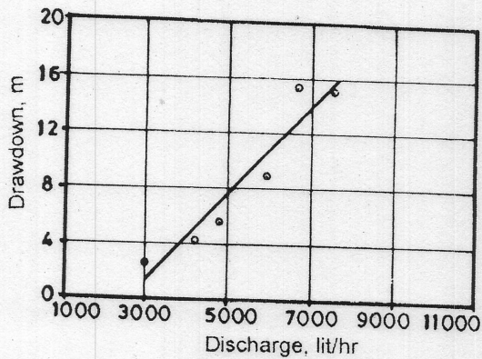
Figure 16 : Discharge vs. Step Drawdown
