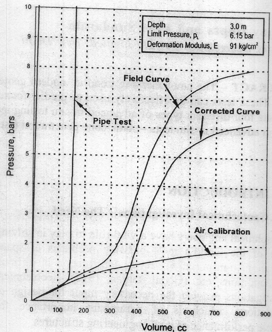
Figure 3 : Typical Results of Pressuremeter Test
