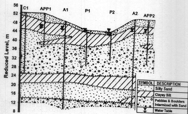
Figure 11 : Interpreted Geo-electric Litholog
