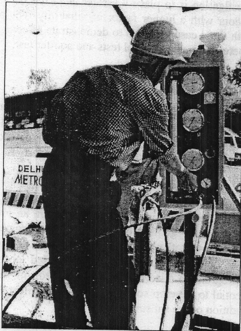
Figure 1 : Pressuremeter Test Setup
