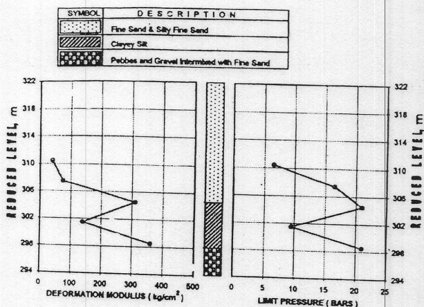
Figure 9 : Profile of Pressuremeter Parameters – Anandpur Sahib
