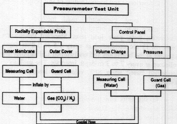
Figure 2 : Pressuremeter Test Schematic
