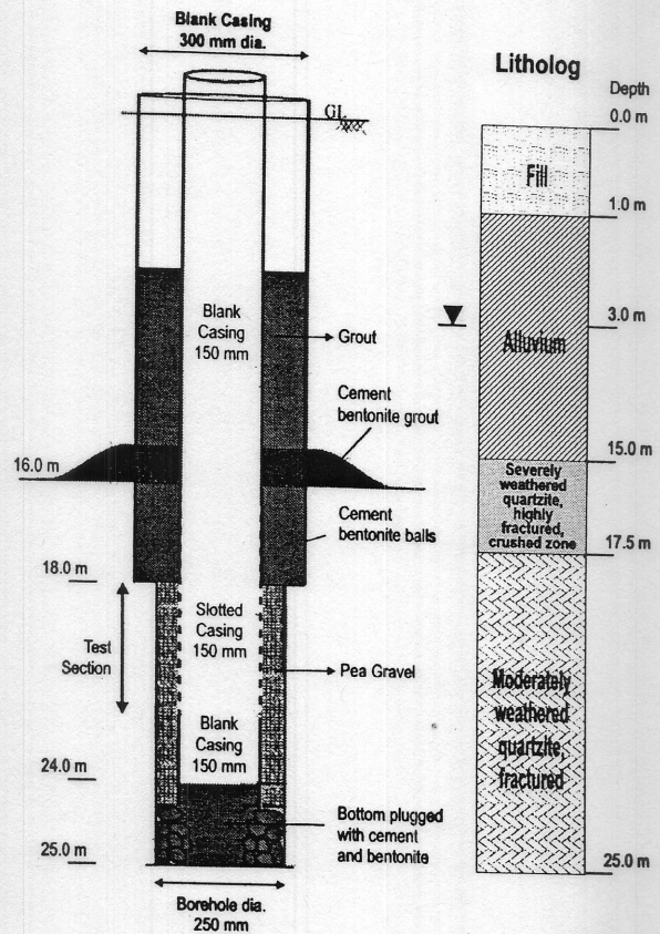
Figure 14 : Pumpwell in Soil-Rock Formation
